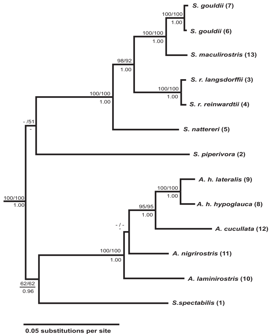
Fig. 2. Maximum likelihood phylogram. Values above nodes are maximum parsimony/maximum likelihood bootstrap values and those below nodes are Bayesian posterior probabilities.
