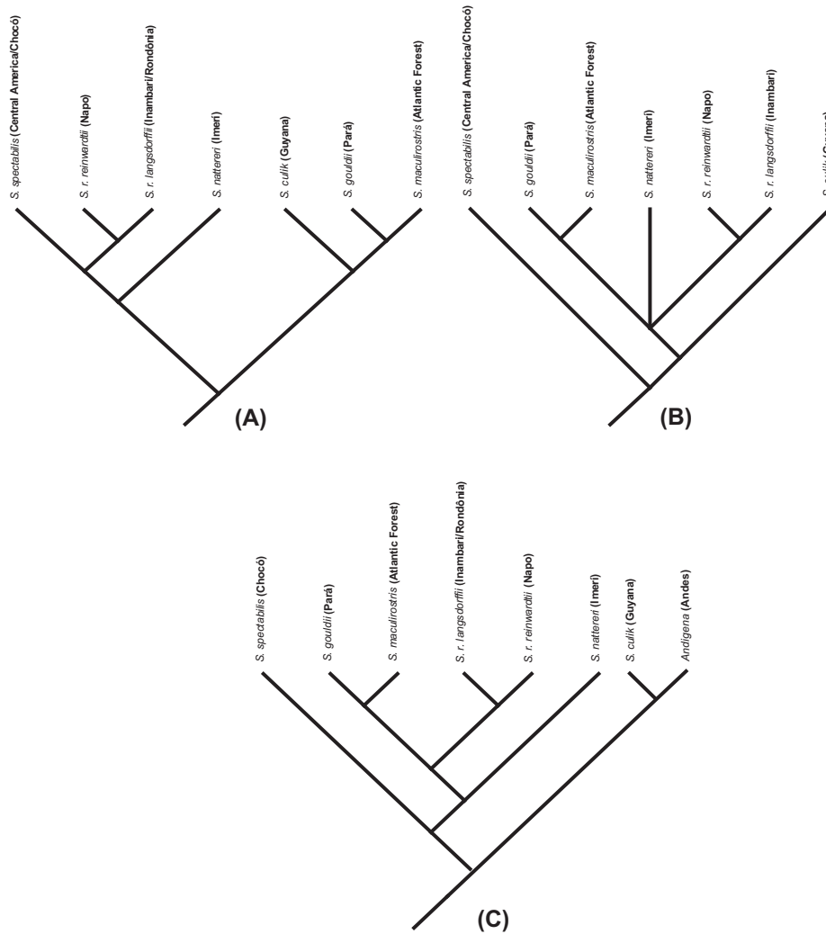
Fig. 4. A comparison the molecular phylogeny of Selenidera and implied area relationships with previously published Selenidera phylogenetic tree topologies and area relationships: (A) dendrogram of Selenidera (Haffer, 1974), (B) morphological phylogeny of Selenidera (Cracraft and Prum, 1988), and (C) molecular phylogeny of Selenidera (this study).
