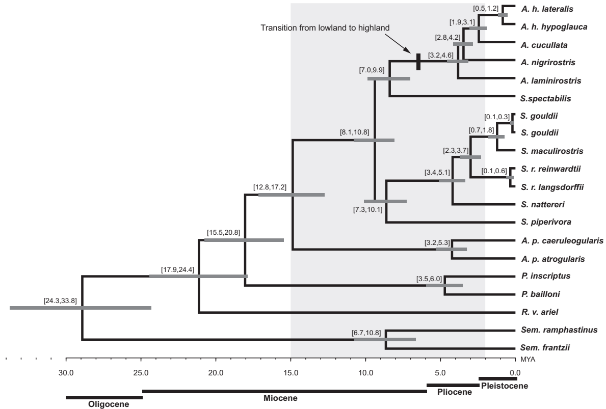
Fig. 3. BEAST chronogram. Horizontal gray bars represent 95% confidence intervals on the median estimates of the timing of maximum divergence events. Vertical gray shading indicates period during which divergences could be attributable to Andean uplift.
