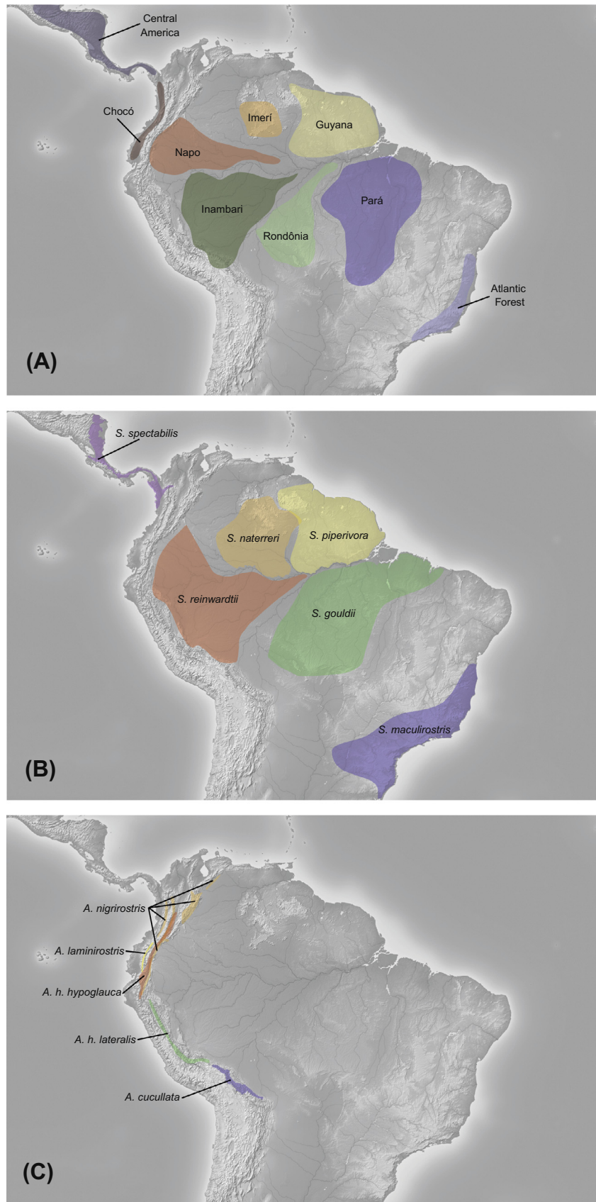
Fig. 1. Approximate distributions of (A) Amazonia areas of endemism, (B) Selenidera species, and (C) Andigena species.
